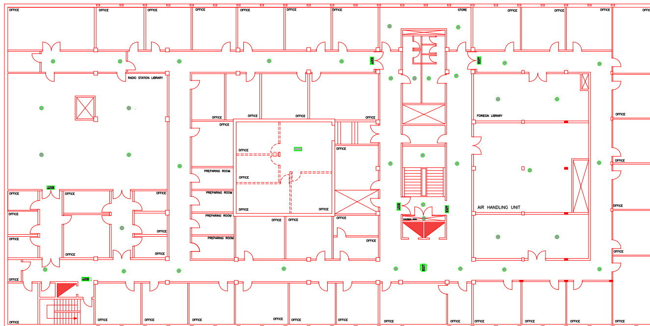
SECOND FLOOR LEVEL (+10.55)
